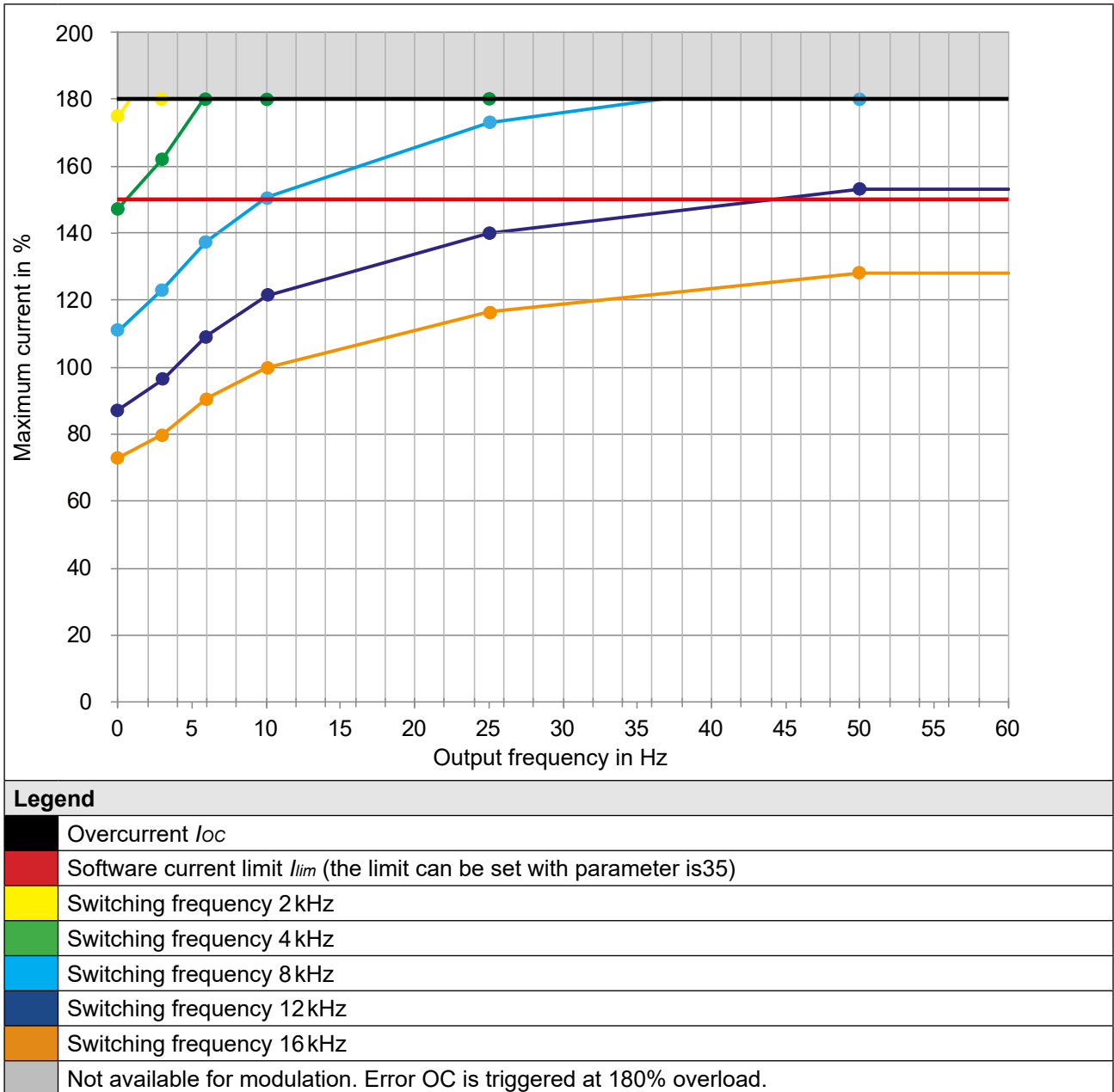
Figure 4: Typical overload characteristics in the lower output frequencies (OL2) Example. Device size 18
